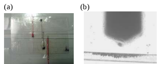
Fig. 2. (a) The microchannel and the small electromagnet wound on a drilling bit core (0.5 mm diameter), (b) the aggregated nanoparticles in the microchannel under the electromagnet.
