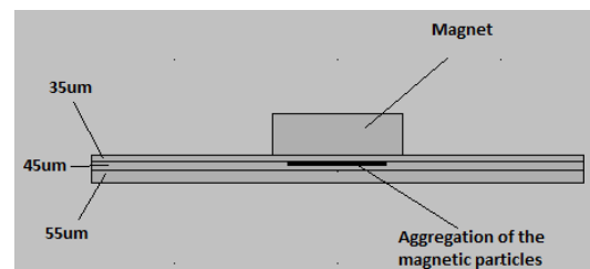
Fig. 1. The schematics of the microchannel system.
