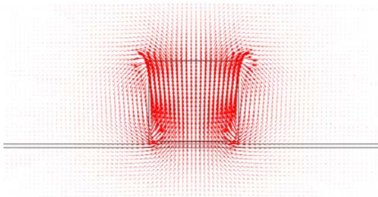
Fig. 3. A 2mm×2mm permanent magnet above the channel and distribution of the magnetic field.
